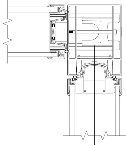
"X" Post Detail
