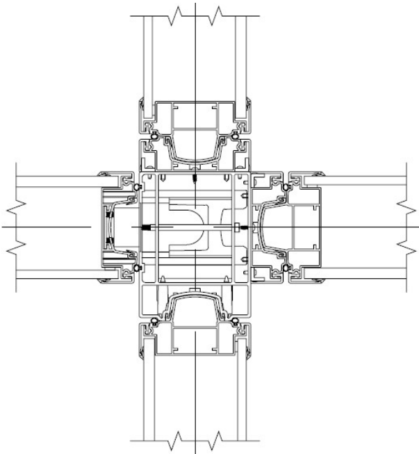
"X" Post Detail
