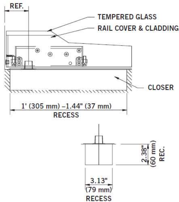
BTS 80 Door Closer
