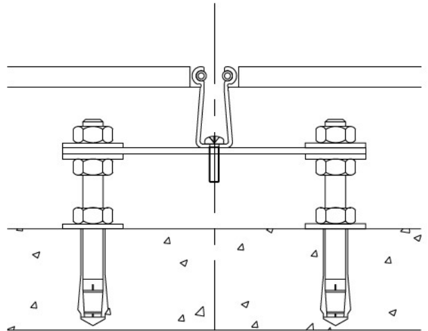
Recessed Floor Guide – Elevated
